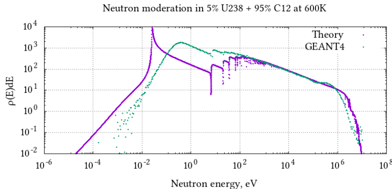
Figure 1: Energy spectrum of the moderating neutrons in uranium-carbon medium (5% ^{238}\text{U} + 95% C) calculated using Eq. (5) (Theory) and using GEANT4 software. The initial spectrum was that of fission (6). The medium temperature is 600 K.
