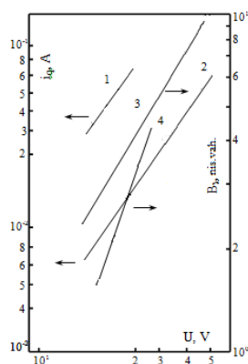
Figure 2. Volt-Amper (1, 2) and Volt-bright (3, 4) characteristics in n-InSe single crystals, doped by Er in a different range. N , at. %: 1, 3 - 10^{-3} ; 2, 4 - 10^{-1} ; T=77K .
